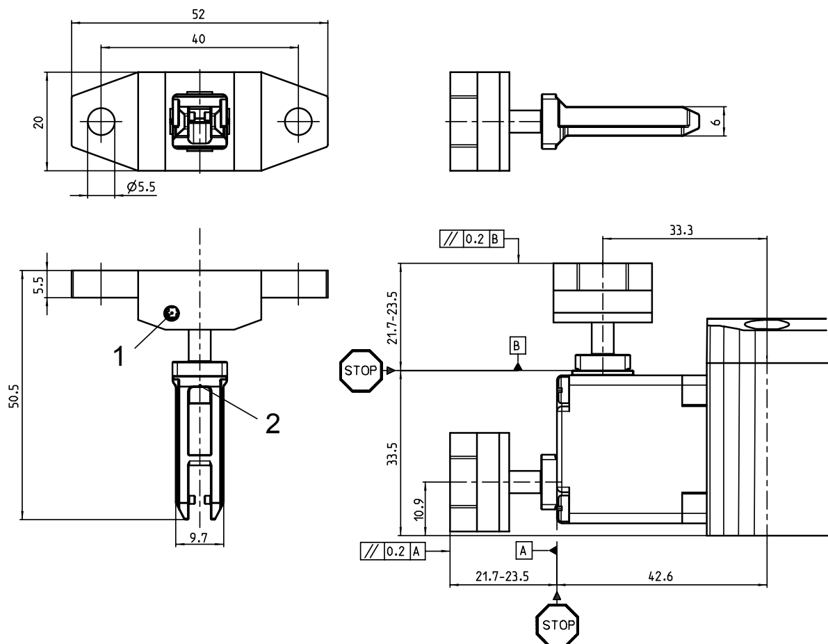
SI-QM-SMFA-2 dimensions
