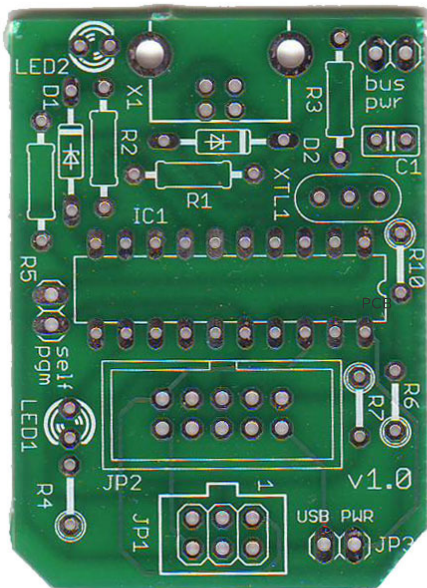
Circuit board
