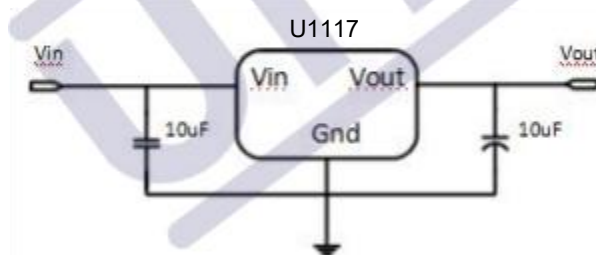
Application circuit of U 1117 fixed version
