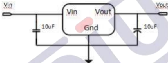
Application circuit of U1117 fixed version
