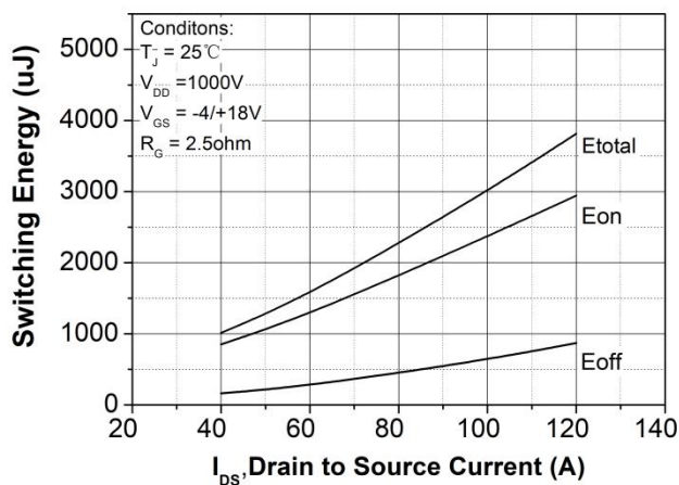
Figure 23. Clamped Inductive switching energy vs. drain current ( V_{DD} = 1000\text{V} )
