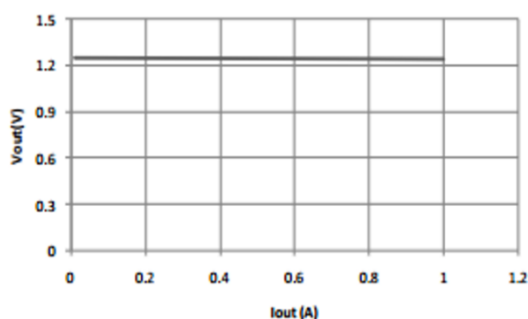
Load regulation JTD1117C-ADJ Vout Vs. Iout
