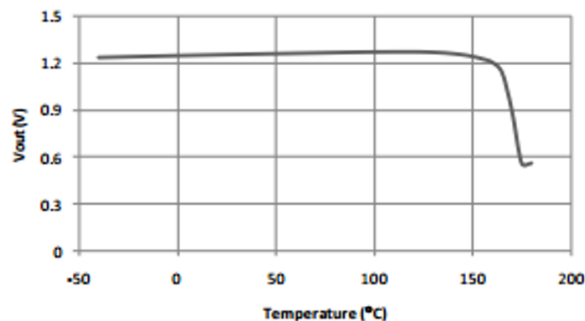
Thermal performance with OTP JTD1117C Thermal performance with OTP
