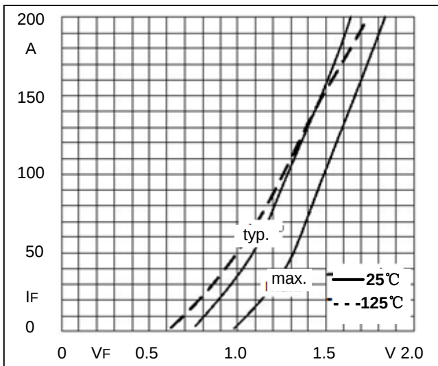
Fig1. Forward Characteristics
