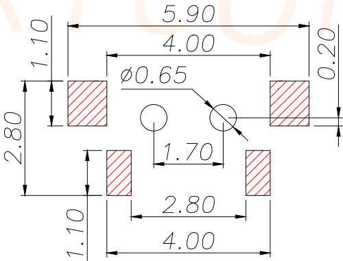
PCB.WELDING DRAWING
