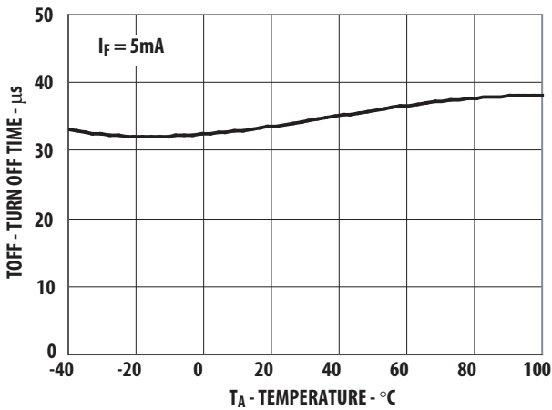
Figure 14: Typical Turn Off Time vs. Temperature
