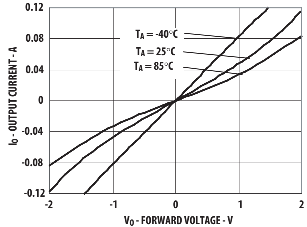
Figure 10: Typical Output Current vs. Output Voltage
