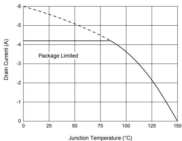
Fig. 2 - Drain Current Characteristics
