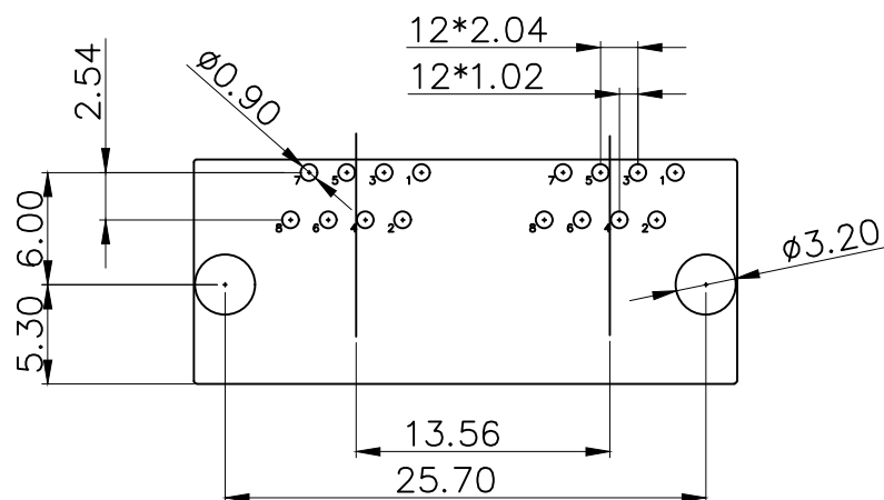
RECOMMENDED PCB LAYOUT TOP VIEW(TOL:±0.05)
