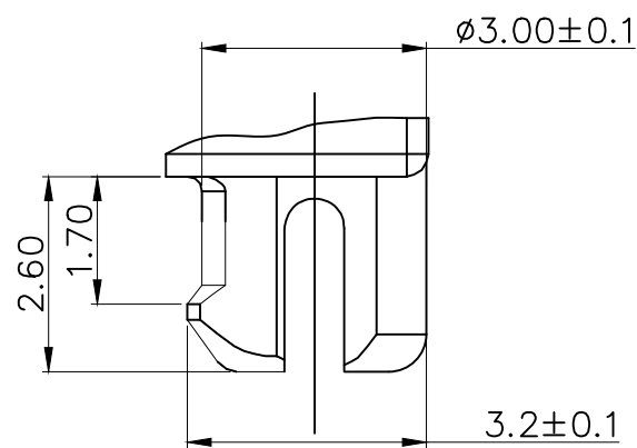
DETAIL "X" SCALE 4:1
