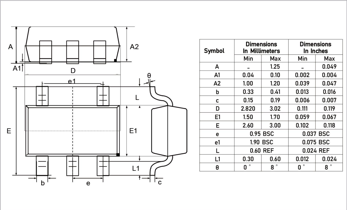
DIMENSIONS, SOT23-5L
