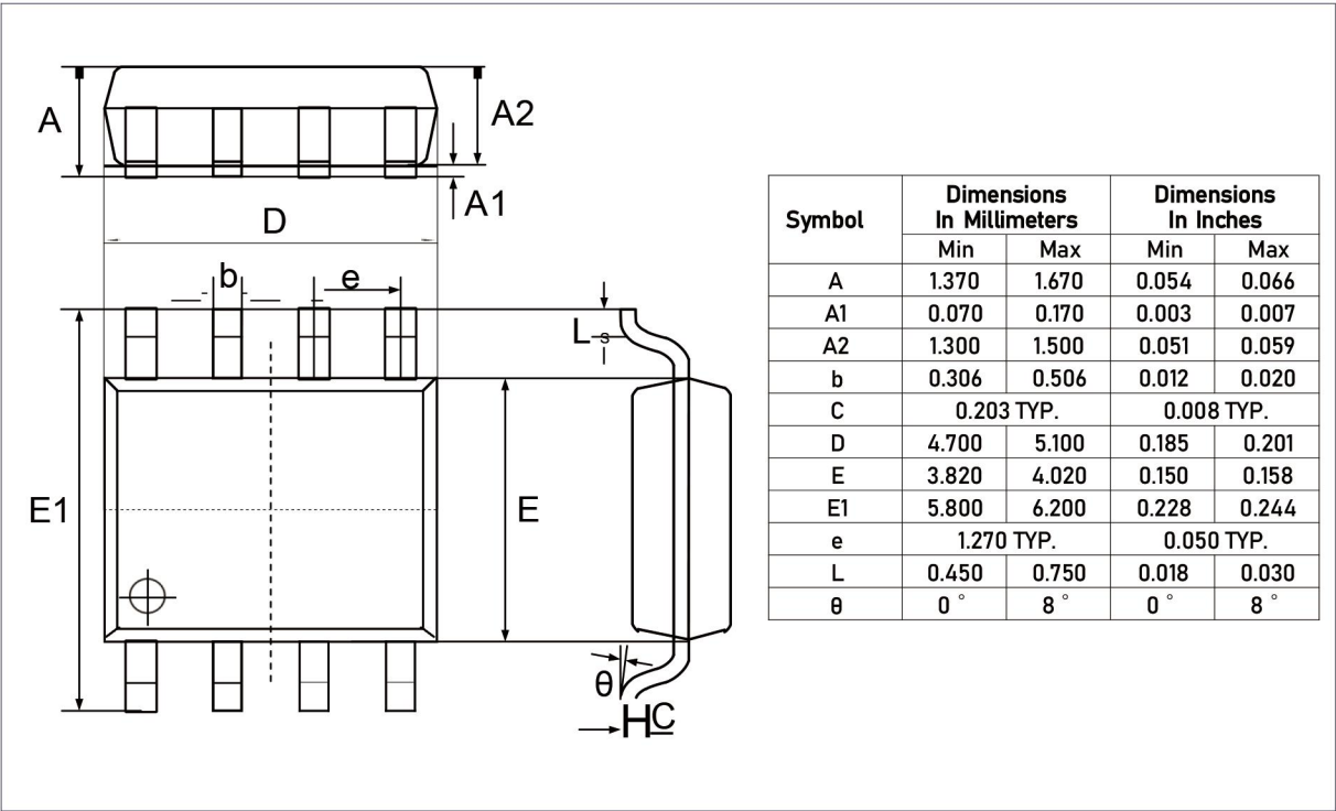
DIMENSIONS, SOIC-8L
